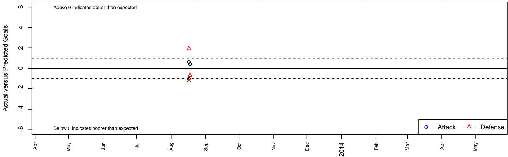
West Coast FC United B01 Dots are actual minus expected GF (blue circles) and GA (red triangles). Blue line is smoothed change in attack strength. Red is smoothed change in defense strength.
